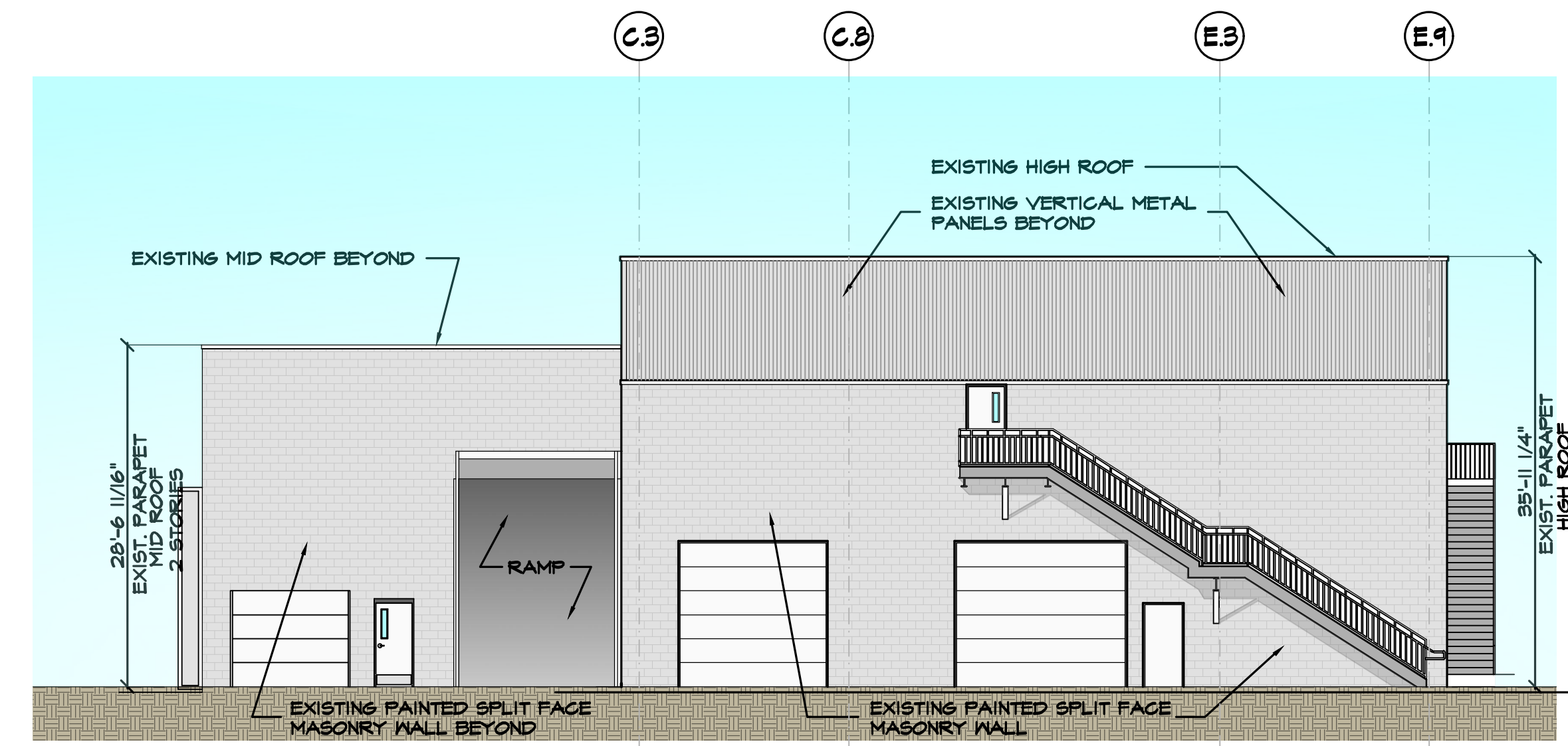
EXISTING REAR (WEST) ELEVATION SCALE 9/32" = 1'-0" 0' 5' 10' 15' 20'
