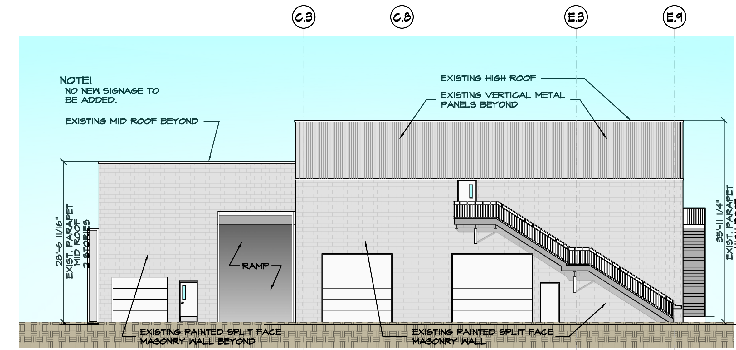
PROPOSED REAR (WEST) ELEVATION SCALE 9/32" = 1'-0" 0' 5' 10' 15' 20'
