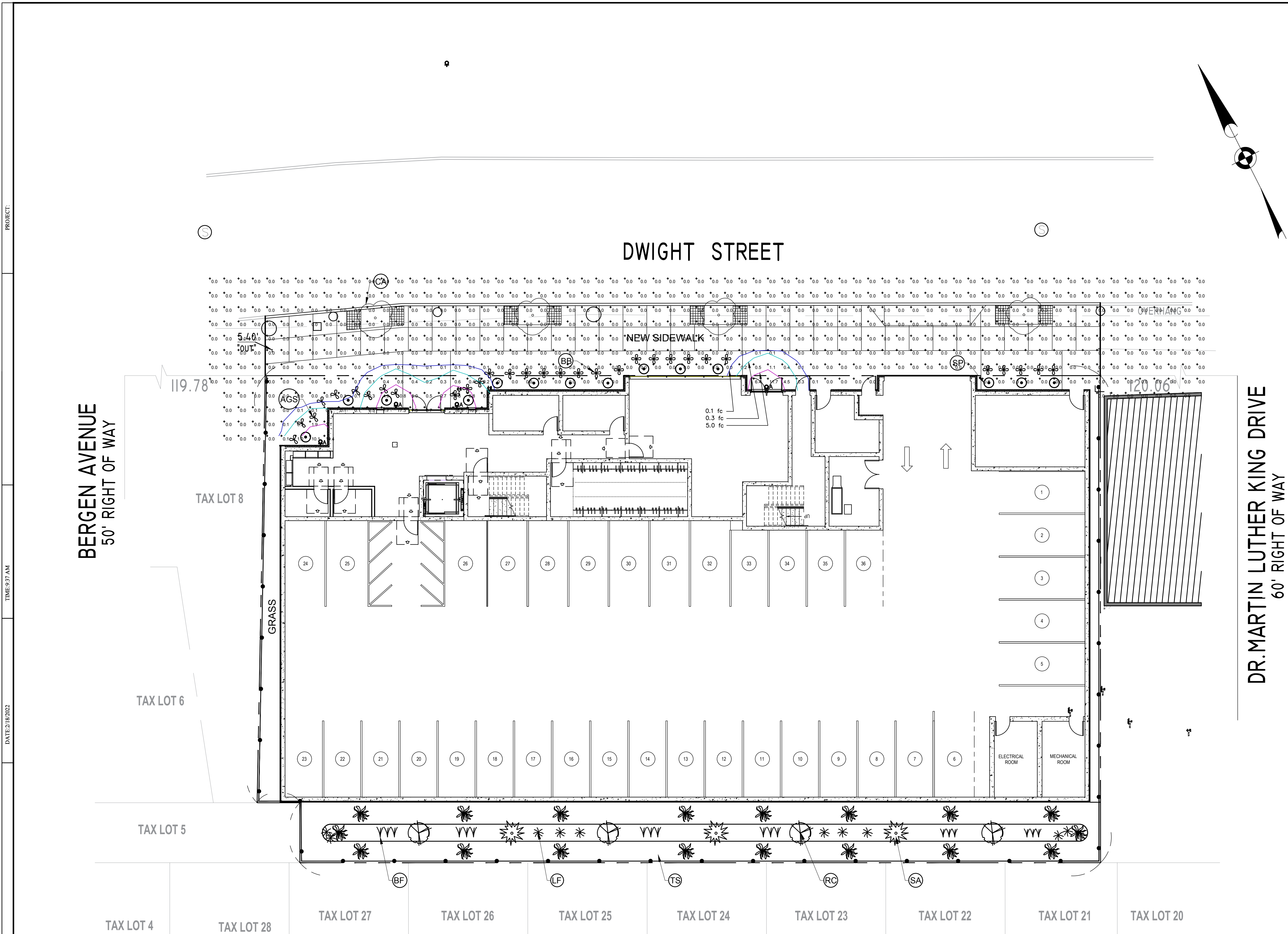
LIGHTING PLAN SCALE: 1"=10'
